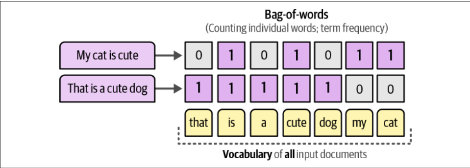
Figure 5-12. A bag-of-words counts the number of times each word appears inside a document.
