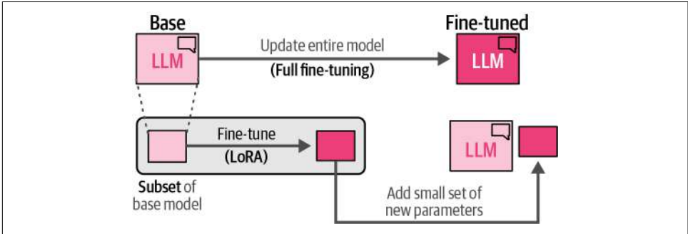
Figure 12-11. LoRA requires only fine-tuning a small set of parameters that can be kept separately from the base LLM.
